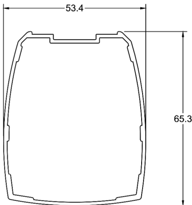
PL-002 Coluna
