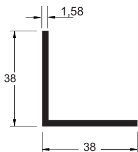
ALM0550 Cantoneira
