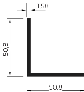
CT-052 Cantoneira 50x50mm
